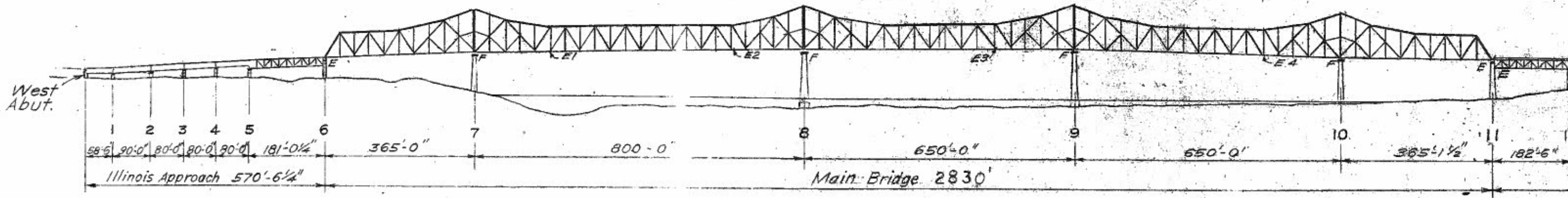
SOUTH PROFILE VIEW
